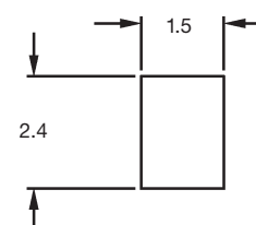
Top PCB Contact Pad (Flash-Gold) Dimensions
