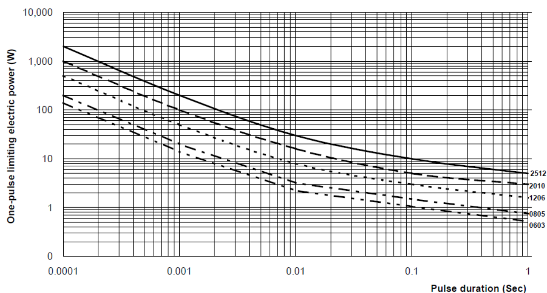
Fig. 13 Maximum permissible peak pulse power as a function of pulse duration
