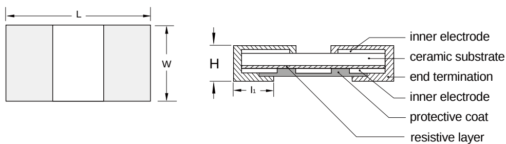
Fig. 10 Chip resistor outlines for PE2512 (3W&5W) / PE2817
