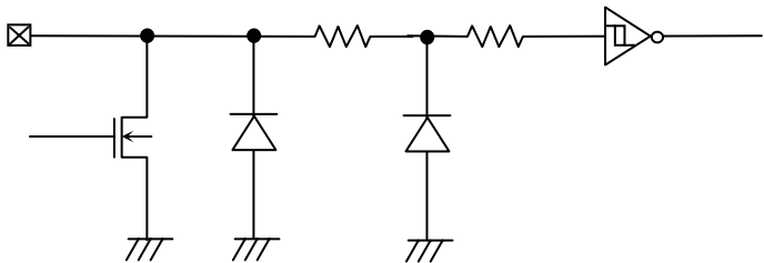
Figure 57. Input / output pin circuit diagram
