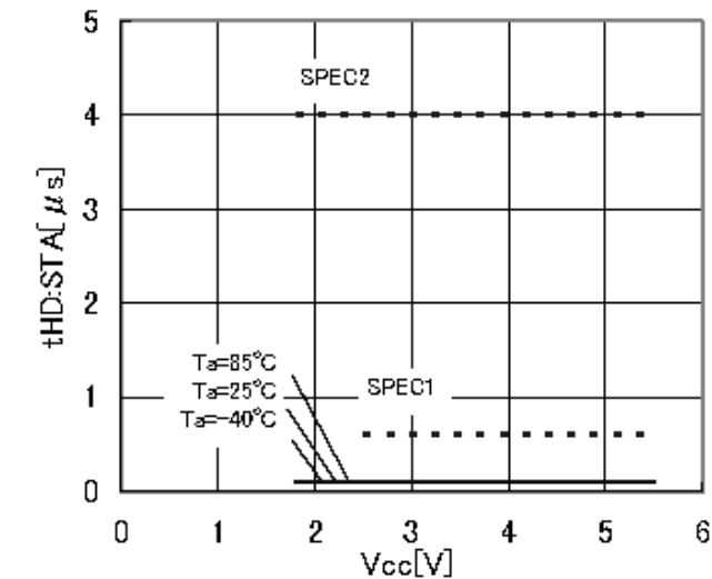
Figure 18. Start condition hold time t_{HD:STA}
