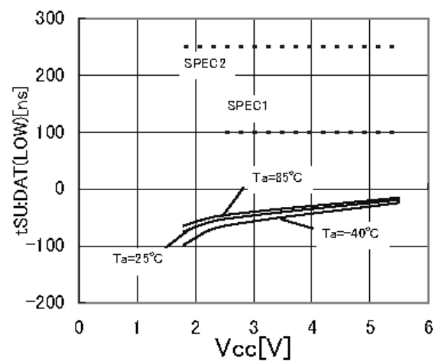
Figure 23. Input data setup time t_{SU:DAT(LOW)}
