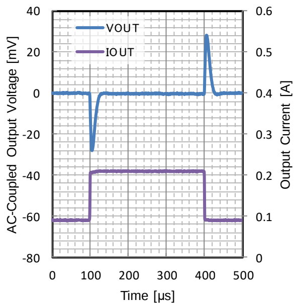
Figure 100. Load Transient
