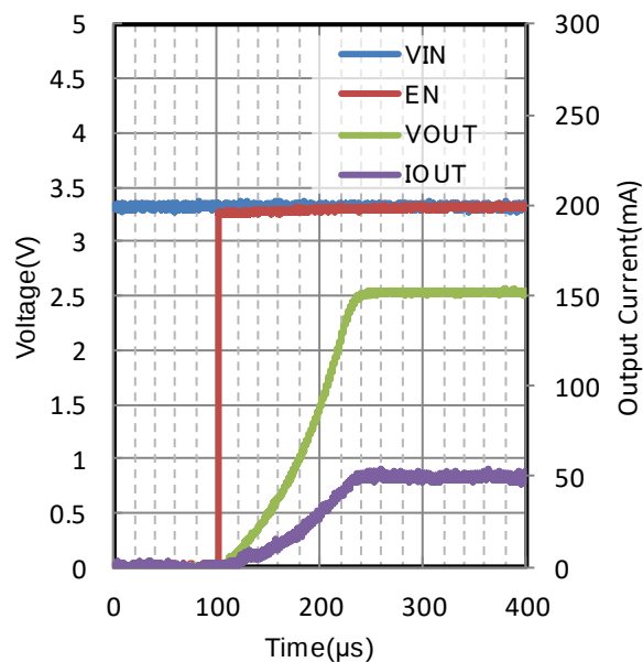
Figure 166. Start Up Waveform V_{OUT} = 2.5\text{ V} , I_{OUT} = 50\text{ mA} V_{IN} = 3.3\text{ V} , C_{OUT} = 10\text{ }\mu\text{F} T_j = 25\text{ }^{\circ}\text{C}
