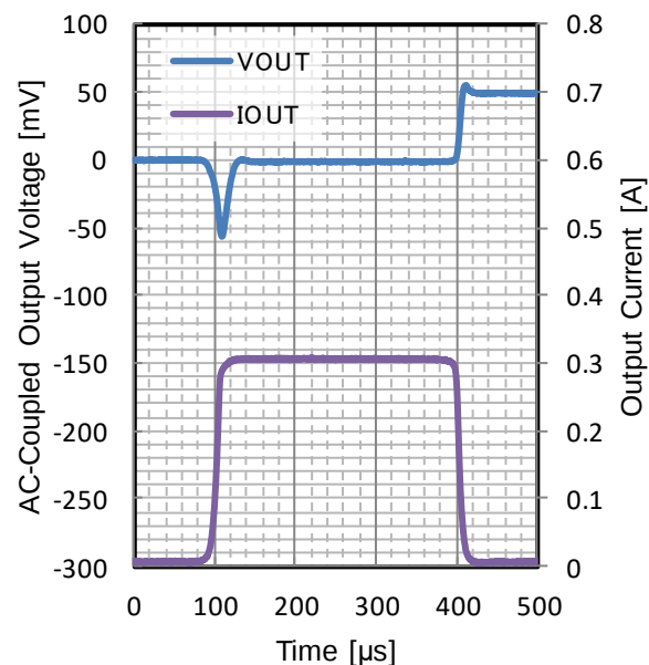
Figure 104. Load Transient
