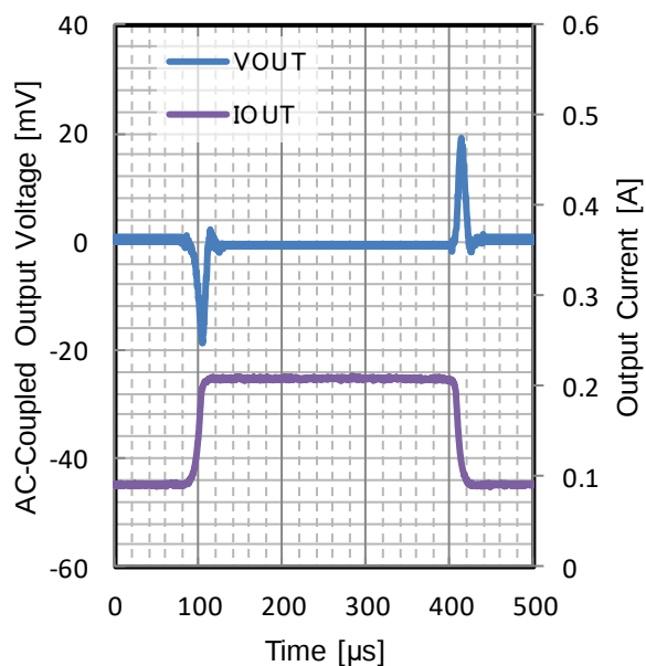
Figure 24. Load Transient
