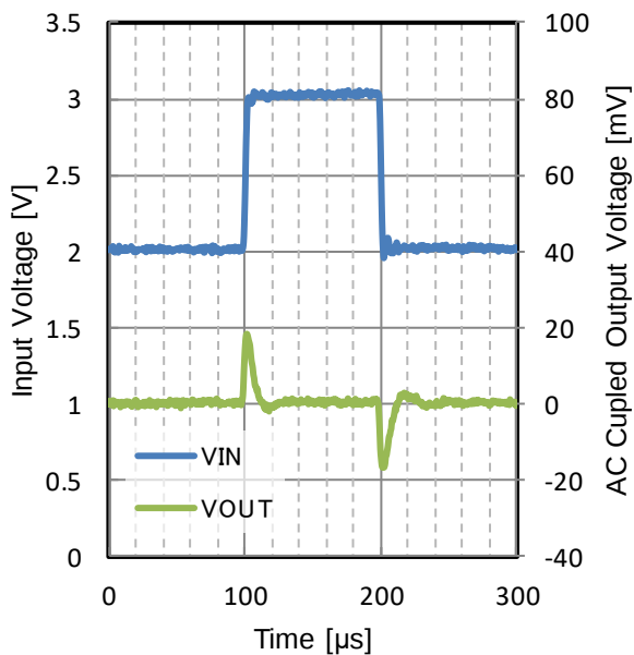
Figure 69. Line Transient
