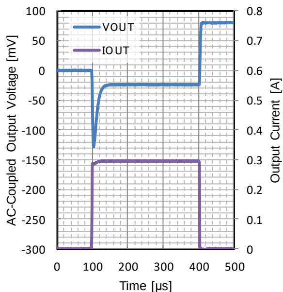
Figure 185. Load Transient
