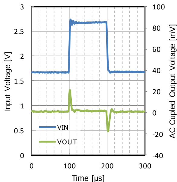
Figure 34. Line Transient V_{OUT} = 1.2\text{ V} t_R = t_F = 1\text{ V}/\mu\text{s} , I_{OUT} = 300\text{ mA} , C_{OUT} = 10\text{ }\mu\text{F} T_J = 25\text{ }^\circ\text{C}
