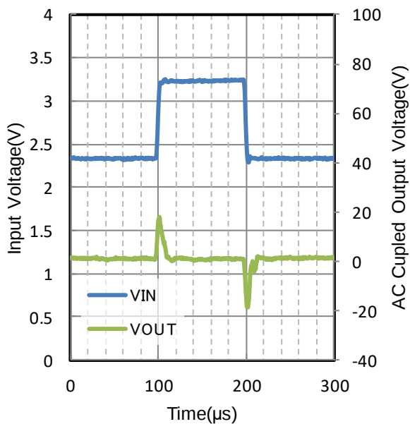
Figure 119. Line Transient
