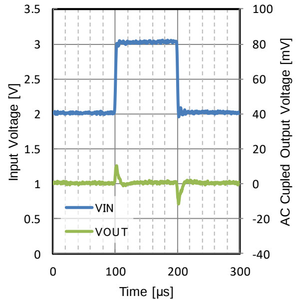
Figure 68. Line Transient
