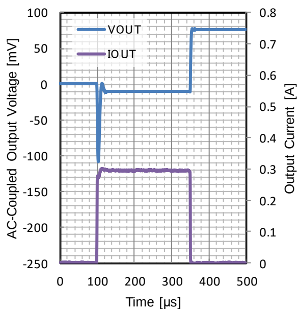
Figure 15. Load Transient
