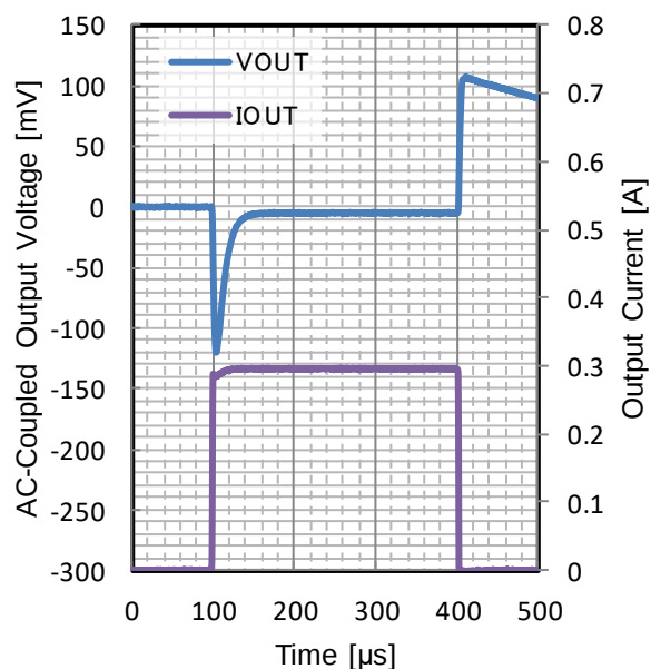
Figure 227. Load Transient
