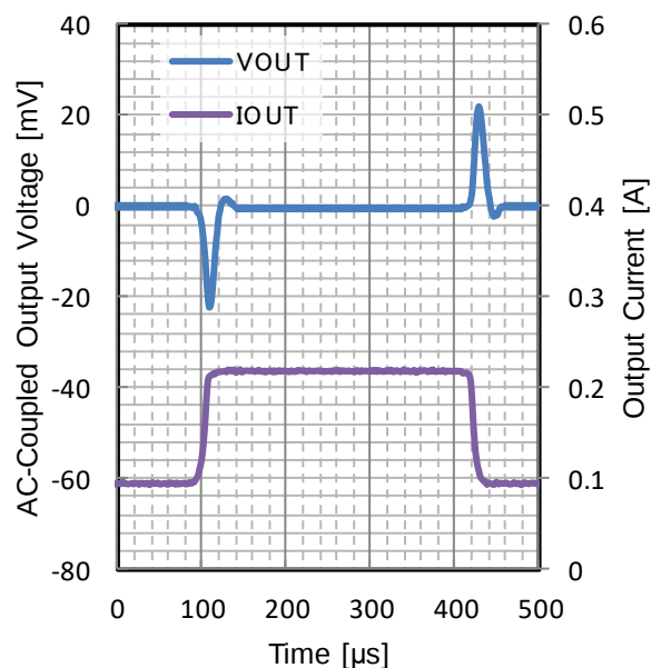
Figure 65. Load Transient
