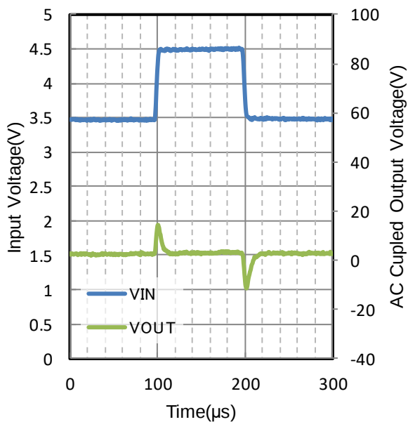
Figure 207. Line Transient
