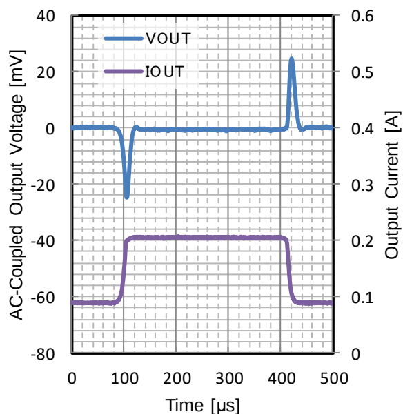
Figure 108. Load Transient
