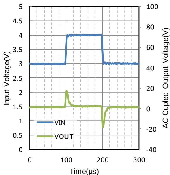
Figure 164. Line Transient V_{OUT} = 2.5\text{ V} t_R = t_F = 1\text{ V}/\mu\text{s} , I_{OUT} = 300\text{ mA} , C_{OUT} = 10\text{ }\mu\text{F} T_j = 150\text{ }^\circ\text{C}
