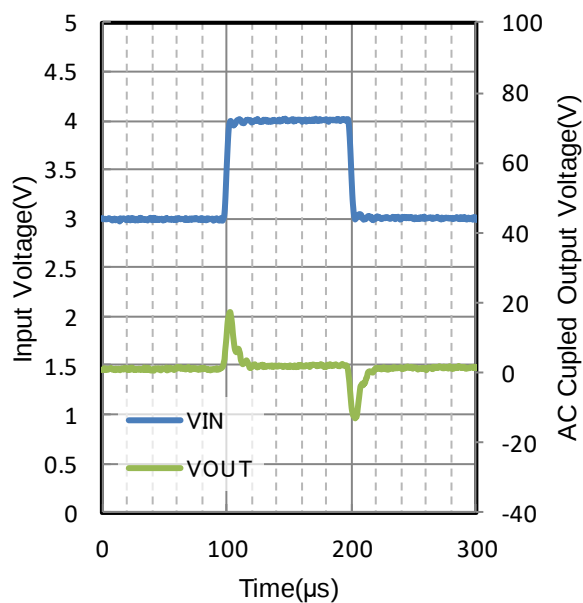
Figure 160. Line Transient V_{OUT} = 2.5\text{ V} t_R = t_F = 1\text{ V}/\mu\text{s} , I_{OUT} = 100\text{ mA} , C_{OUT} = 10\text{ }\mu\text{F} T_j = 150\text{ }^\circ\text{C}
