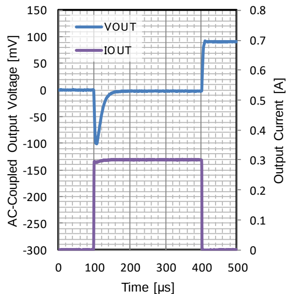
Figure 225. Load Transient
