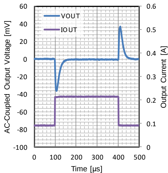
Figure 229. Load Transient
