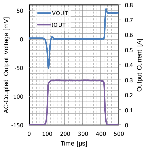
Figure 62. Load Transient
