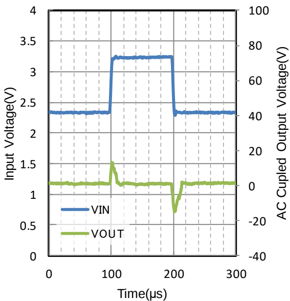
Figure 111. Line Transient
