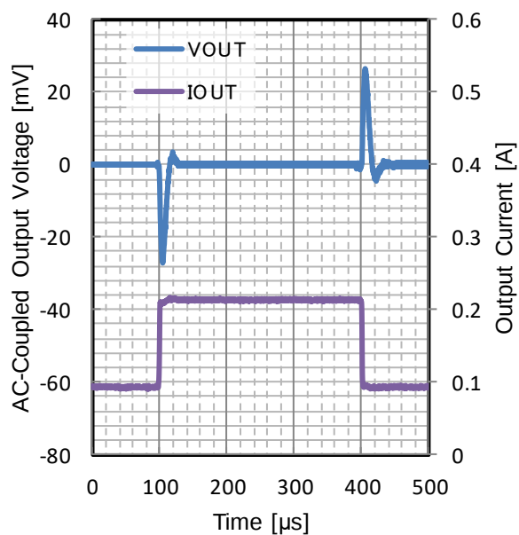
Figure 16. Load Transient
