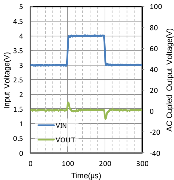
Figure 158. Line Transient V_{OUT} = 2.5\text{ V} t_R = t_F = 1\text{ V}/\mu\text{s} , I_{OUT} = 100\text{ mA} , C_{OUT} = 10\text{ }\mu\text{F} T_j = 25\text{ }^\circ\text{C}
