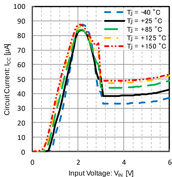
Figure 172. Circuit Current vs Input Voltage V_{OUT} = 3.0\text{ V}
