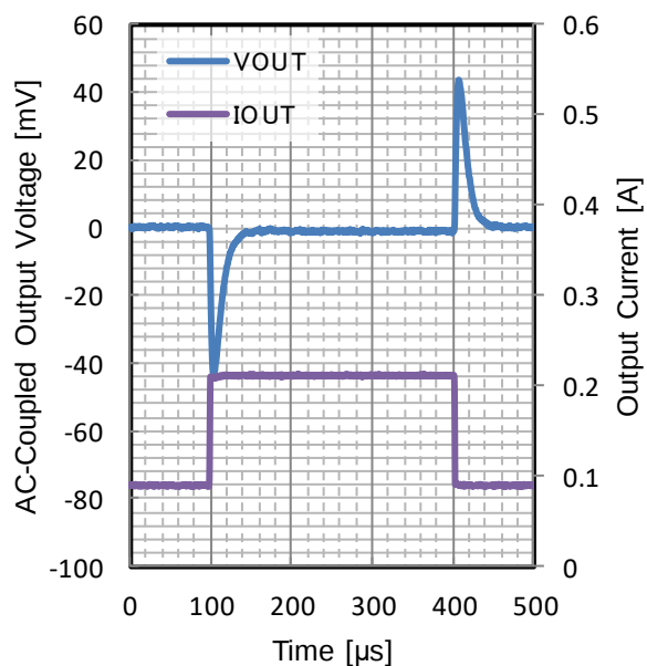
Figure 230. Load Transient
