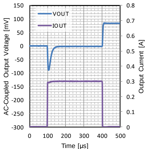
Figure 184. Load Transient
