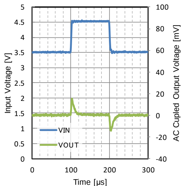
Figure 200. Line Transient
