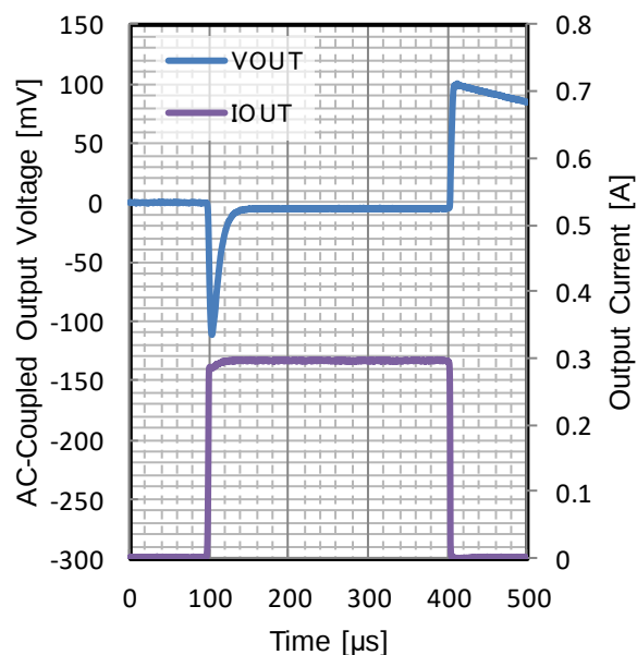
Figure 186. Load Transient
