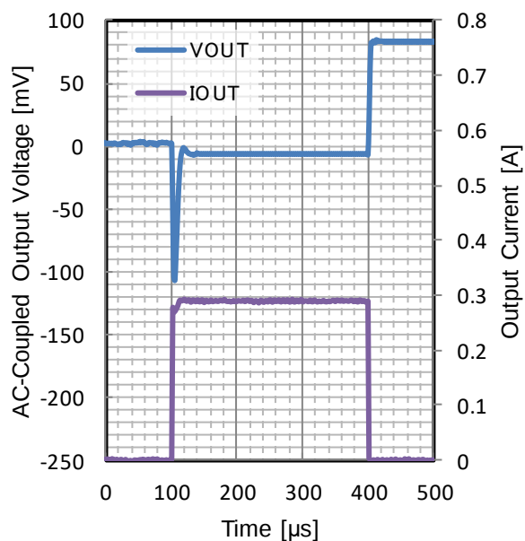
Figure 57. Load Transient
