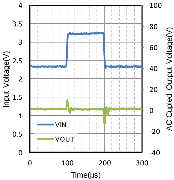
Figure 117. Line Transient
