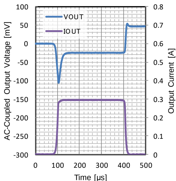
Figure 192. Load Transient
