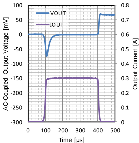
Figure 190. Load Transient
