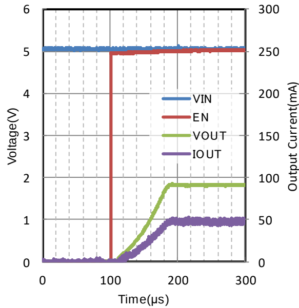
Figure 125. Start Up Waveform V_{OUT} = 1.8\text{ V} , I_{OUT} = 50\text{ mA} V_{IN} = 5.0\text{ V} , C_{OUT} = 10\text{ }\mu\text{F} T_j = 25\text{ }^{\circ}\text{C}
