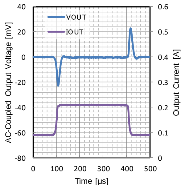
Figure 107. Load Transient
