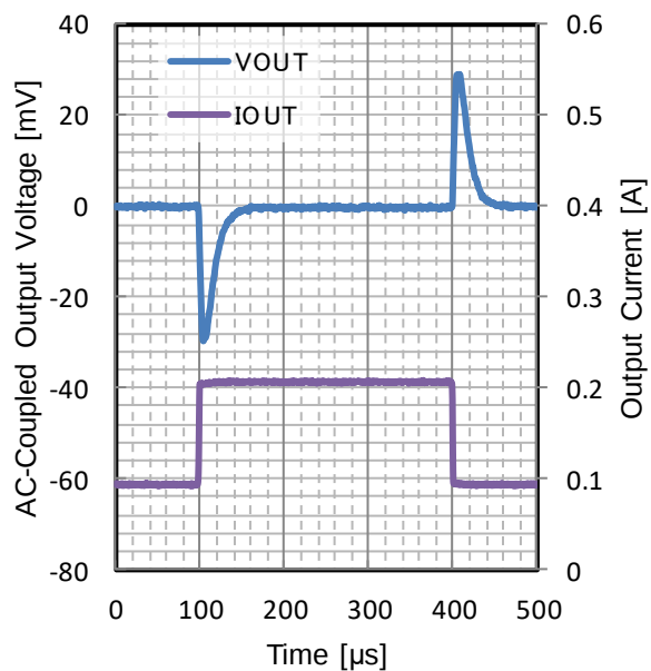
Figure 143. Load Transient
