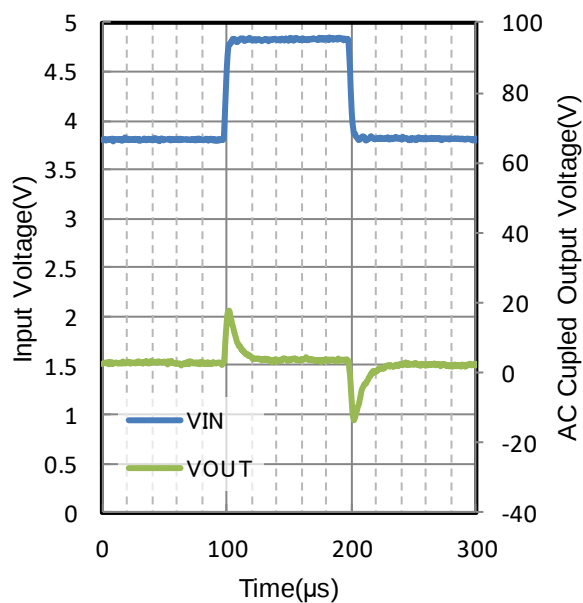
Figure 245. Line Transient
