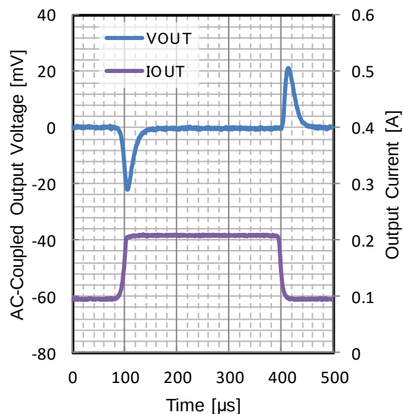
Figure 195. Load Transient
