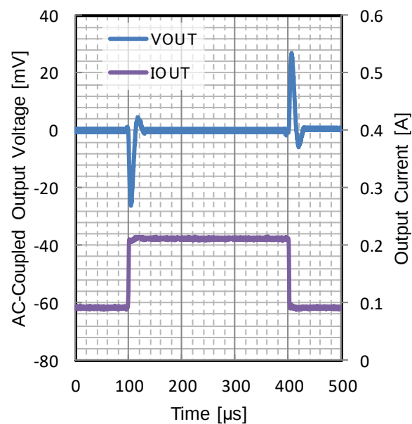
Figure 17. Load Transient
