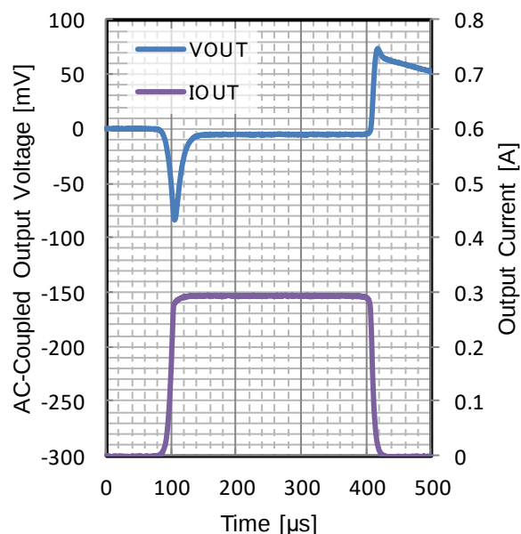
Figure 193. Load Transient
