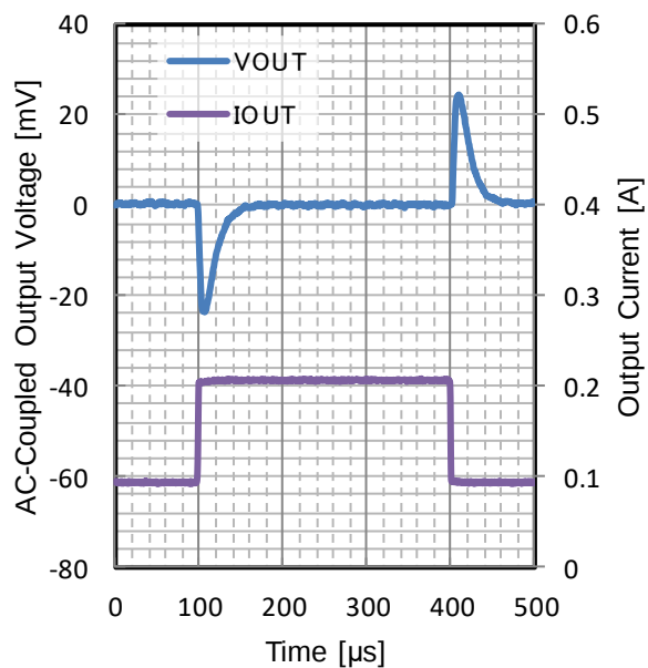
Figure 187. Load Transient
