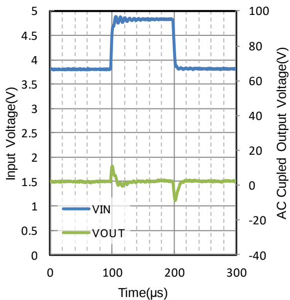
Figure 242. Line Transient
