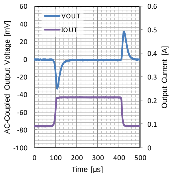
Figure 236. Load Transient
