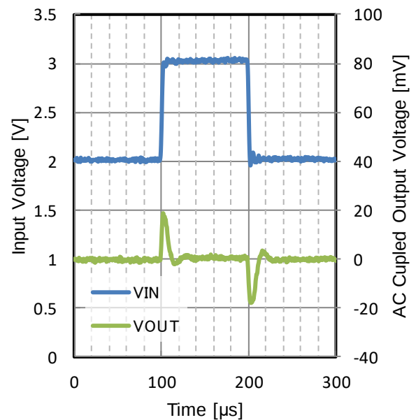
Figure 70. Line Transient
