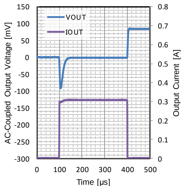
Figure 140. Load Transient V_{OUT} = 2.5\text{ V}
