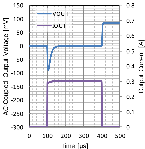
Figure 139. Load Transient V_{OUT} = 2.5\text{ V}
