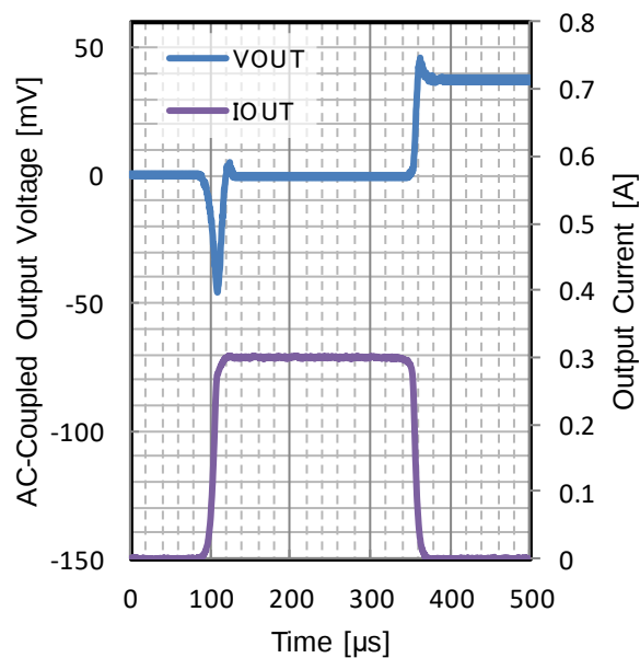
Figure 20. Load Transient
