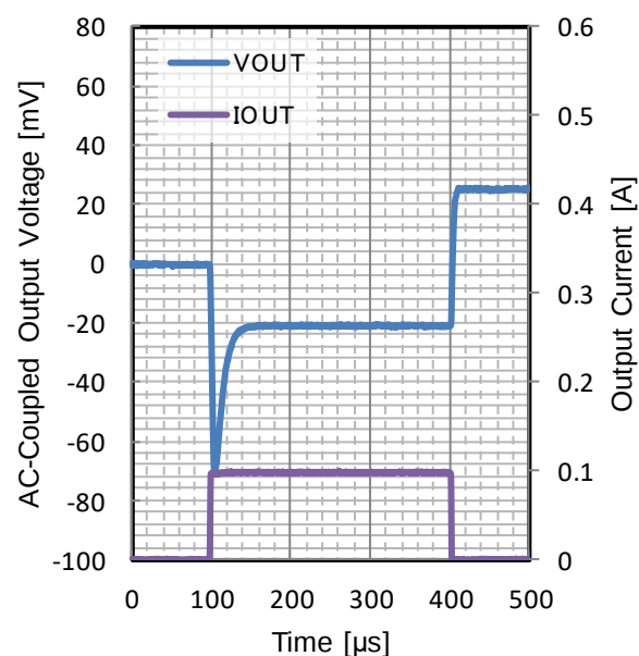
Figure 223. Load Transient V_{OUT} = 3.3\text{ V} t_R = t_F = 1\text{ }\mu\text{s} , I_{OUT} = 0\text{ mA to }100\text{ mA} , C_{OUT} = 10\text{ }\mu\text{F} T_j = 150\text{ }^\circ\text{C}
