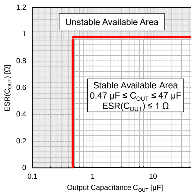
Figure 261. Output Capacitance C_{OUT} , ESR Stable Available Area (-40 °C ≤ T j ≤ +150 °C, 1.7 V ≤ V IN ≤ 6.5 V, V EN = 1.5 V, I OUT = 0 mA to 300 mA)
