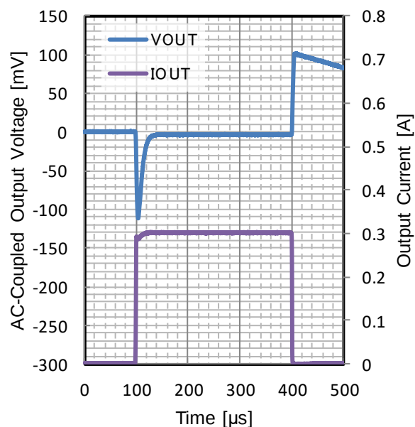
Figure 142. Load Transient V_{OUT} = 2.5\text{ V}
