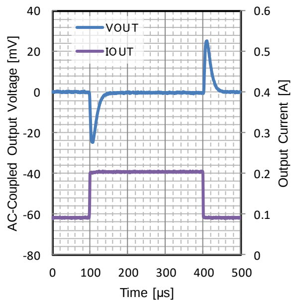
Figure 188. Load Transient
