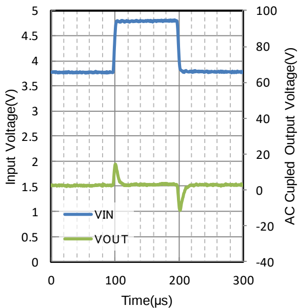
Figure 248. Line Transient
