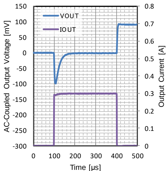
Figure 224. Load Transient
