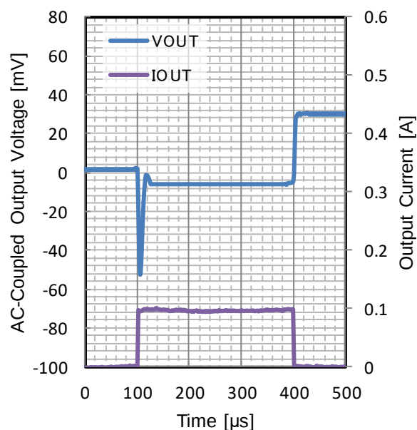
Figure 54. Load Transient V_{OUT} = 1.5\text{ V} t_R = t_F = 1\text{ }\mu\text{s} , I_{OUT} = 0\text{ mA to }100\text{ mA} , C_{OUT} = 10\text{ }\mu\text{F} T_j = 150\text{ }^\circ\text{C}
