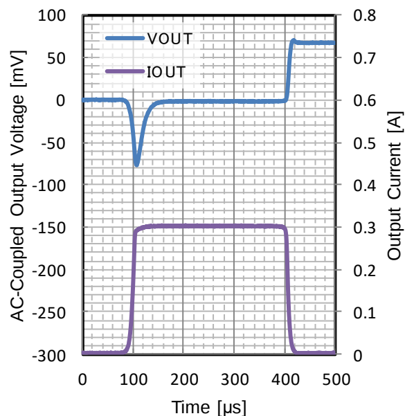
Figure 191. Load Transient
