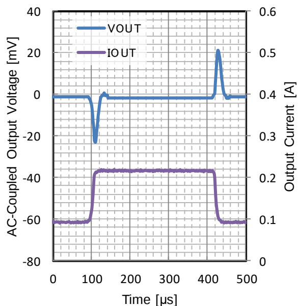
Figure 64. Load Transient
