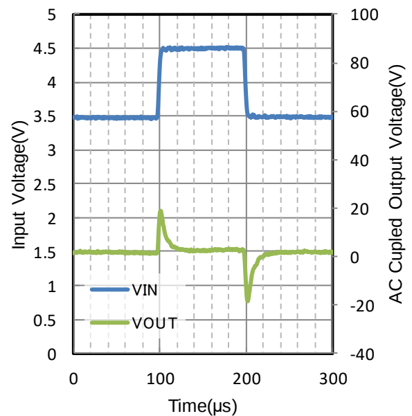
Figure 208. Line Transient
