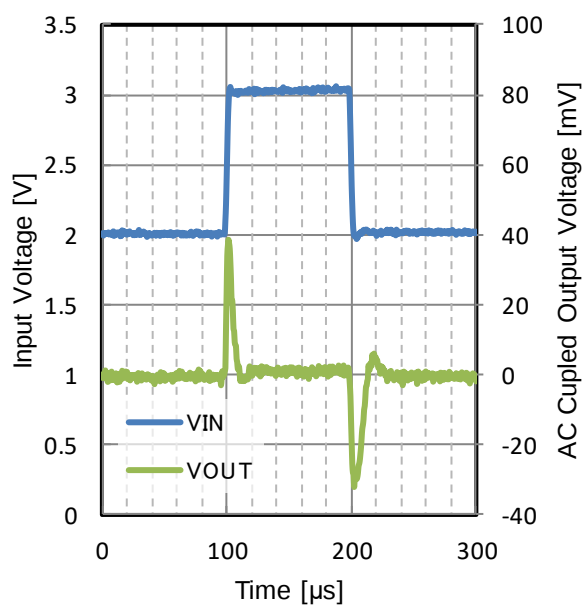
Figure 78. Line Transient V_{OUT} = 1.5\text{ V} t_R = t_F = 1\text{ V}/\mu\text{s} , I_{OUT} = 300\text{ mA} , C_{OUT} = 10\text{ }\mu\text{F} T_J = 150\text{ }^\circ\text{C}
