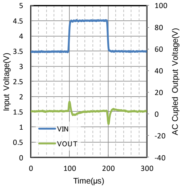
Figure 205. Line Transient
