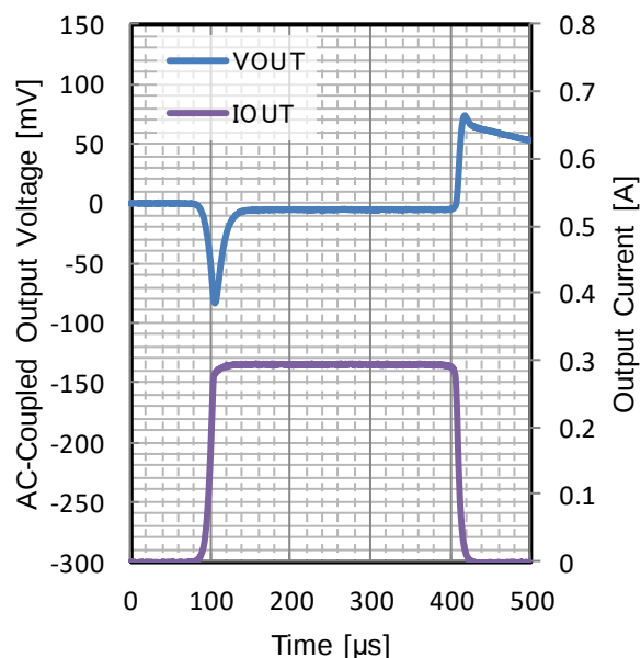
Figure 234. Load Transient
