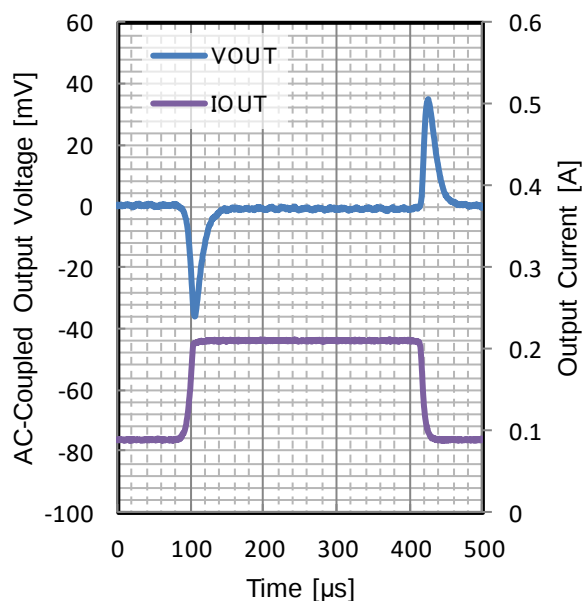
Figure 237. Load Transient
