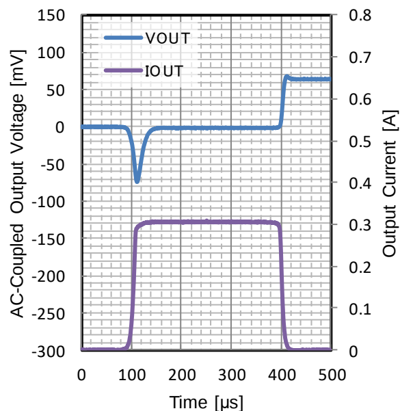
Figure 147. Load Transient
