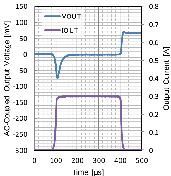
Figure 231. Load Transient
