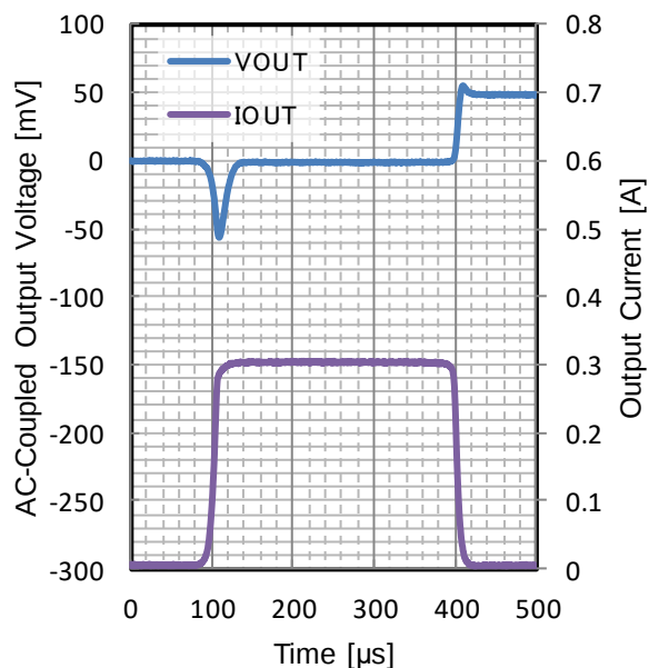
Figure 103. Load Transient
