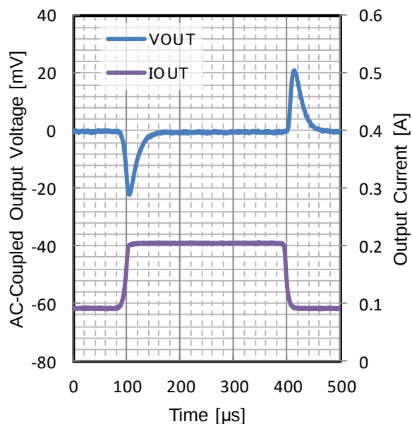
Figure 194. Load Transient
