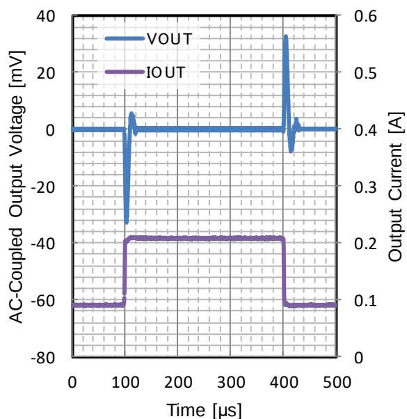
Figure 18. Load Transient
