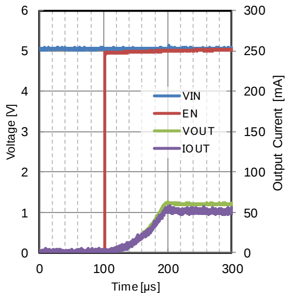
Figure 40. Start Up Waveform V_{OUT} = 1.2\text{ V} , I_{OUT} = 50\text{ mA} V_{IN} = 5.0\text{ V} , C_{OUT} = 10\text{ }\mu\text{F} T_j = -40\text{ }^{\circ}\text{C}
