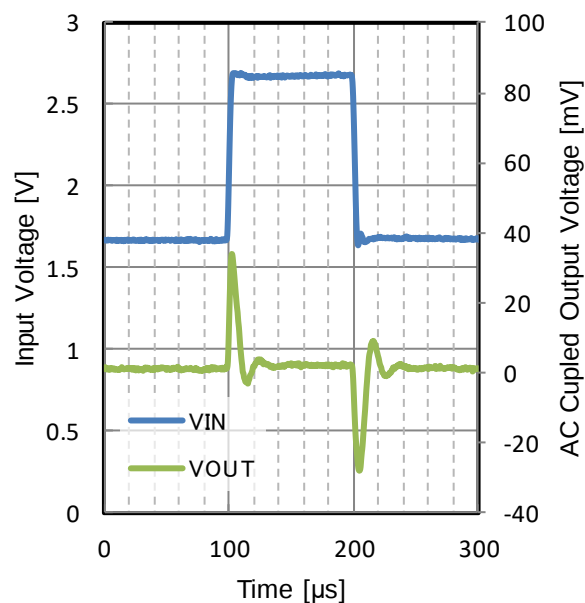
Figure 28. Line Transient V_{OUT} = 1.2\text{ V} t_R = t_F = 1\text{ V}/\mu\text{s} , I_{OUT} = 50\text{ mA} , C_{OUT} = 10\text{ }\mu\text{F} T_J = 150\text{ }^\circ\text{C}
