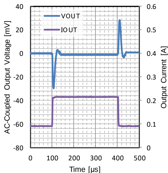
Figure 59. Load Transient
