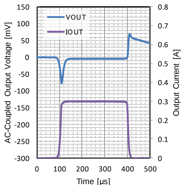
Figure 149. Load Transient
