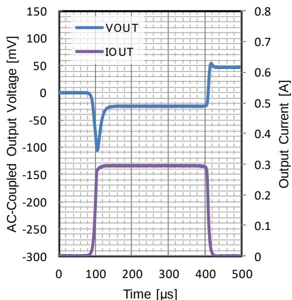
Figure 233. Load Transient
