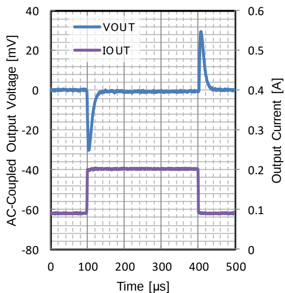
Figure 189. Load Transient
