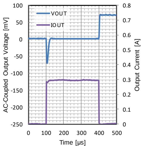
Figure 55. Load Transient
