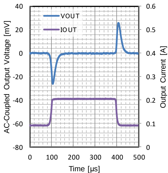
Figure 150. Load Transient
