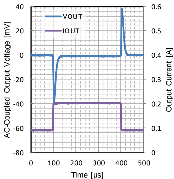
Figure 145. Load Transient
