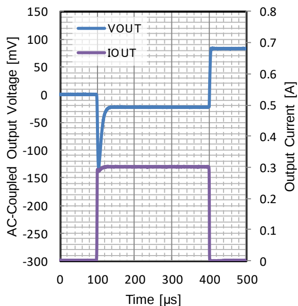
Figure 141. Load Transient V_{OUT} = 2.5\text{ V}
