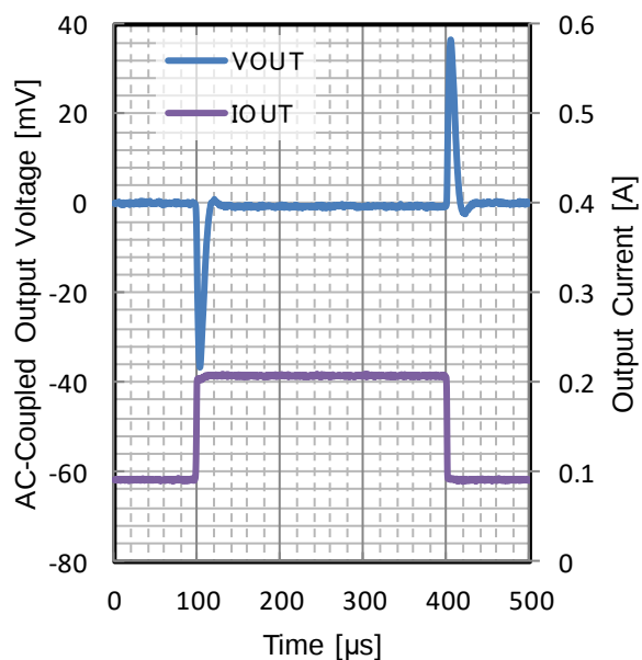
Figure 102. Load Transient
