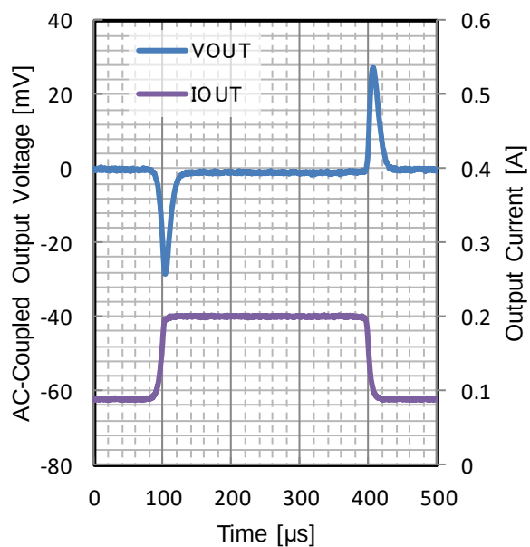
Figure 152. Load Transient
