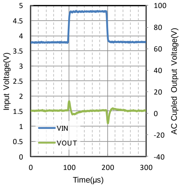
Figure 246. Line Transient
