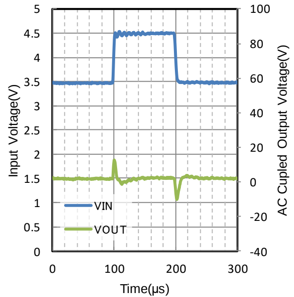
Figure 206. Line Transient
