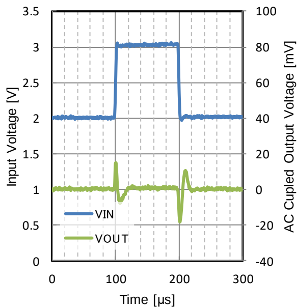
Figure 76. Line Transient V_{OUT} = 1.5\text{ V} t_R = t_F = 1\text{ V}/\mu\text{s} , I_{OUT} = 300\text{ mA} , C_{OUT} = 10\text{ }\mu\text{F} T_J = 25\text{ }^\circ\text{C}
