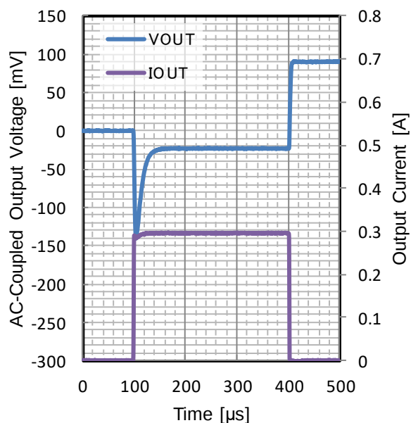
Figure 226. Load Transient
