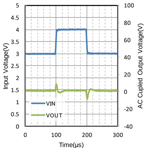
Figure 162. Line Transient V_{OUT} = 2.5\text{ V} t_R = t_F = 1\text{ V}/\mu\text{s} , I_{OUT} = 300\text{ mA} , C_{OUT} = 10\text{ }\mu\text{F} T_j = 25\text{ }^\circ\text{C}
