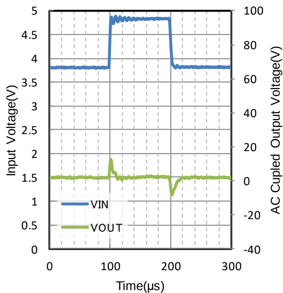
Figure 243. Line Transient
