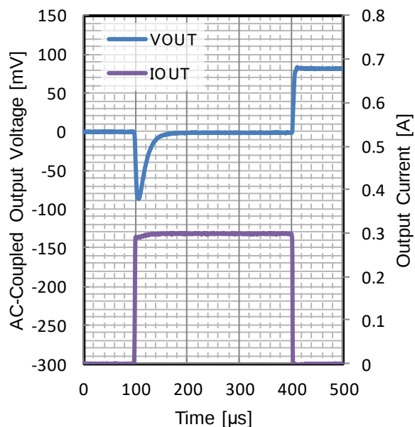
Figure 183. Load Transient
