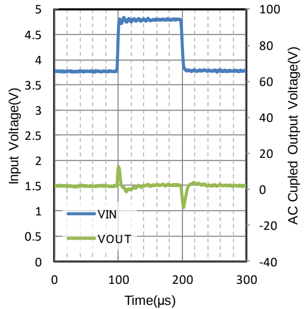
Figure 247. Line Transient
