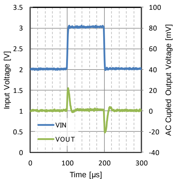
Figure 74. Line Transient V_{OUT} = 1.5\text{ V} t_R = t_F = 1\text{ V}/\mu\text{s} , I_{OUT} = 100\text{ mA} , C_{OUT} = 10\text{ }\mu\text{F} T_j = 150\text{ }^\circ\text{C}
