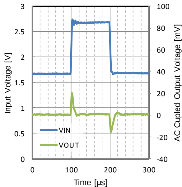
Figure 26. Line Transient V_{OUT} = 1.2\text{ V} t_R = t_F = 1\text{ V}/\mu\text{s} , I_{OUT} = 50\text{ mA} , C_{OUT} = 10\text{ }\mu\text{F} T_J = 25\text{ }^\circ\text{C}
