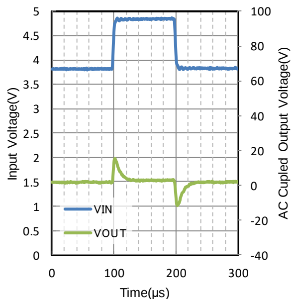
Figure 241. Line Transient
