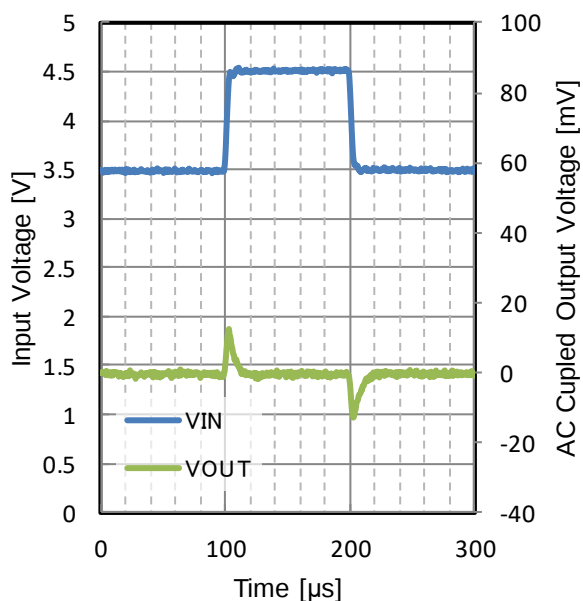
Figure 203. Line Transient
