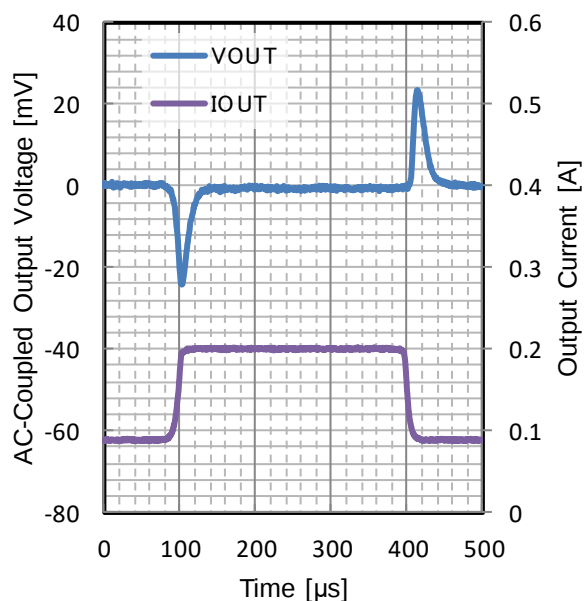
Figure 196. Load Transient
