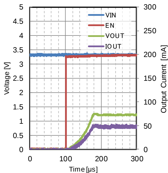
Figure 38. Start Up Waveform V_{OUT} = 1.2\text{ V} , I_{OUT} = 50\text{ mA} V_{IN} = 3.3\text{ V} , C_{OUT} = 10\text{ }\mu\text{F} T_j = 25\text{ }^{\circ}\text{C}
