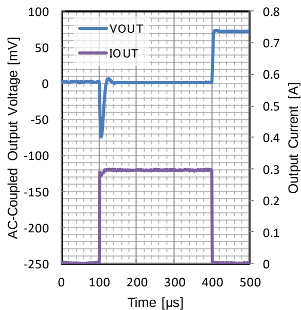
Figure 56. Load Transient
