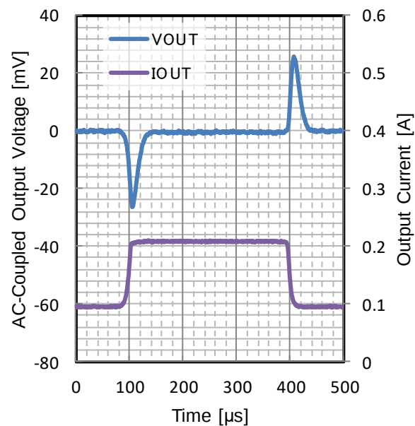
Figure 151. Load Transient
