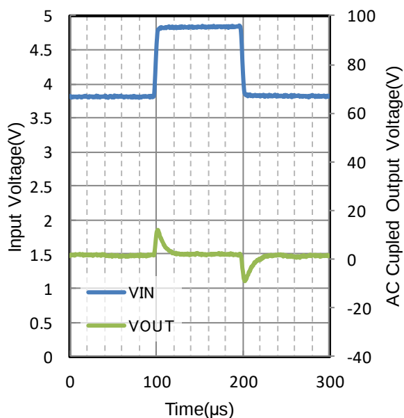
Figure 240. Line Transient
