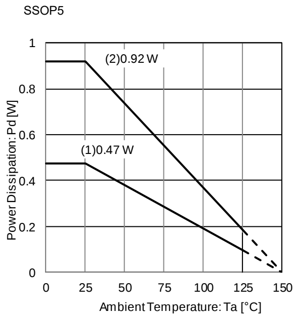
Figure 272. Power Dissipation Graph
