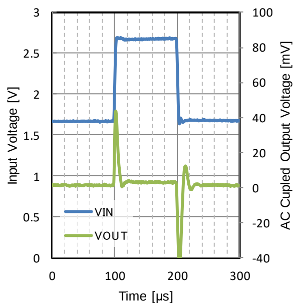
Figure 36. Line Transient V_{OUT} = 1.2\text{ V} t_R = t_F = 1\text{ V}/\mu\text{s} , I_{OUT} = 300\text{ mA} , C_{OUT} = 10\text{ }\mu\text{F} T_J = 150\text{ }^\circ\text{C}
