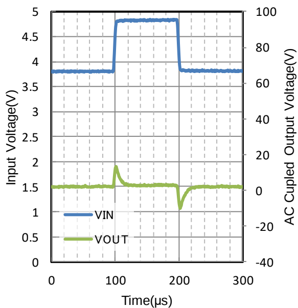
Figure 244. Line Transient
