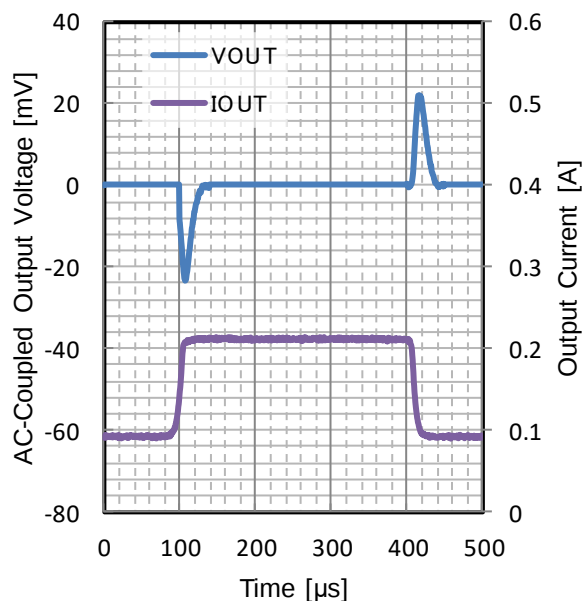
Figure 106. Load Transient
