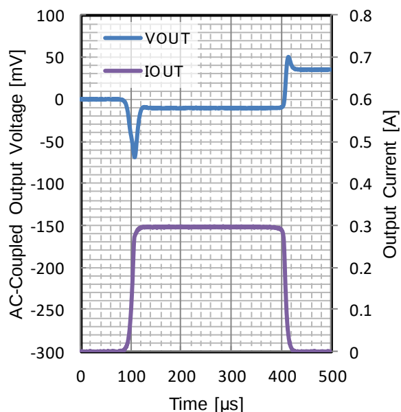
Figure 105. Load Transient
