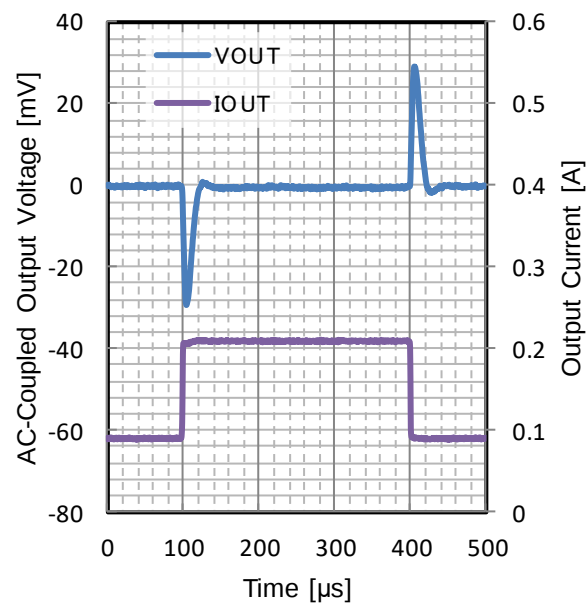
Figure 101. Load Transient
