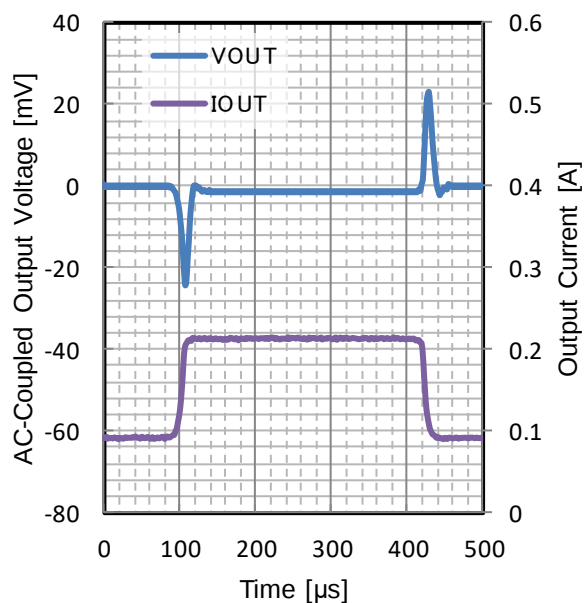
Figure 66. Load Transient
