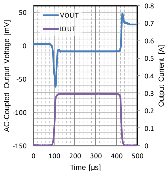
Figure 63. Load Transient
