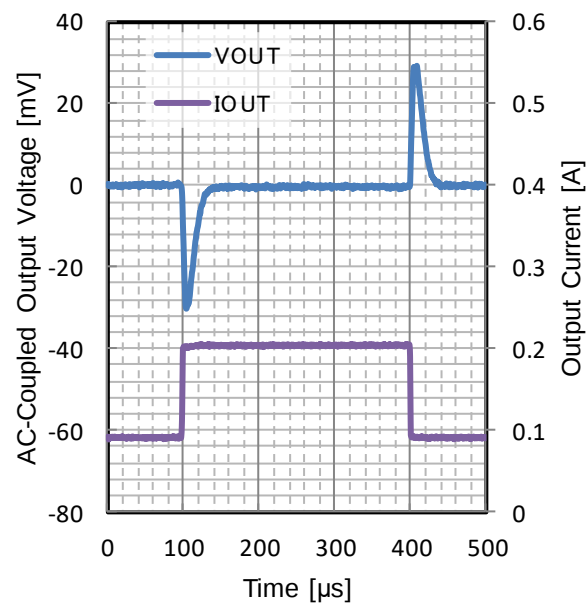
Figure 144. Load Transient
