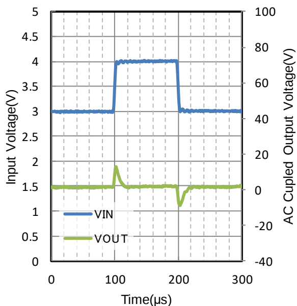
Figure 155. Line Transient
