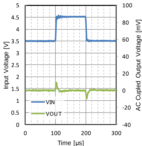
Figure 198. Line Transient
