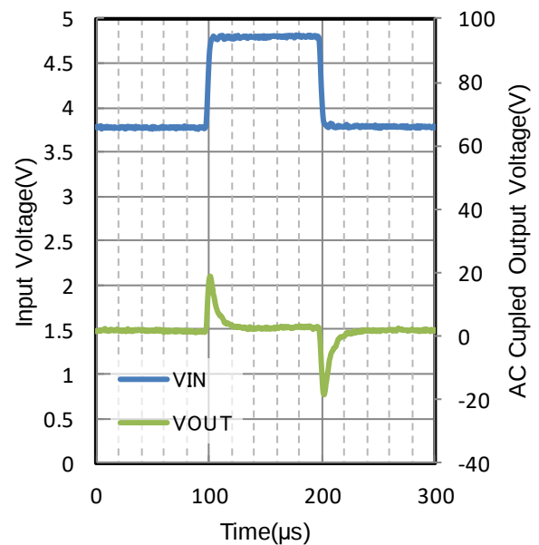
Figure 249. Line Transient
