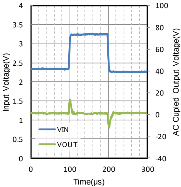
Figure 109. Line Transient
