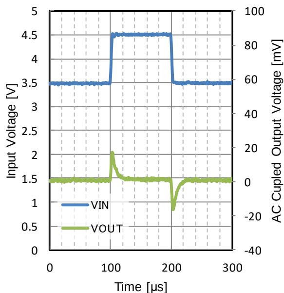
Figure 204. Line Transient
