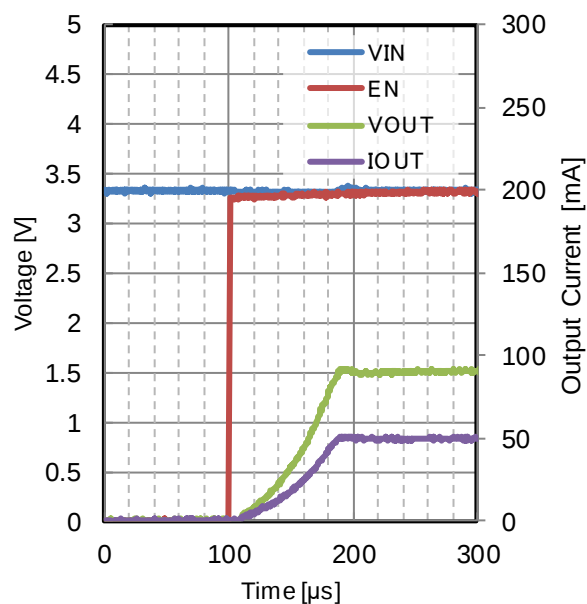
Figure 80. Start Up Waveform V_{OUT} = 1.5\text{ V} , I_{OUT} = 50\text{ mA} V_{IN} = 3.3\text{ V} , C_{OUT} = 10\text{ }\mu\text{F} T_j = 25\text{ }^{\circ}\text{C}
