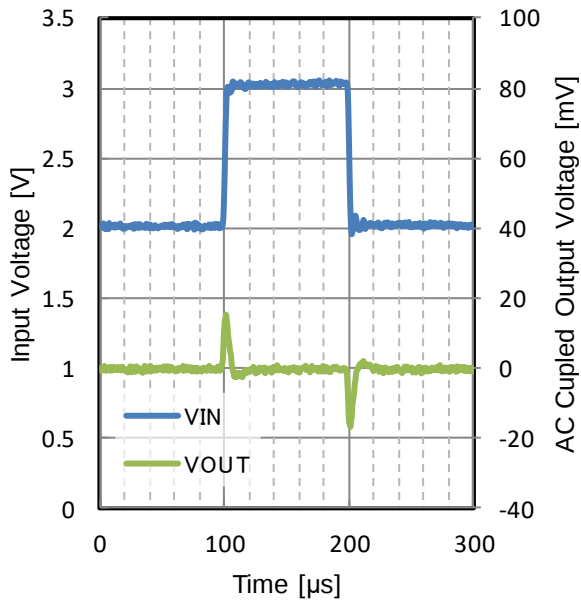
Figure 67. Line Transient
