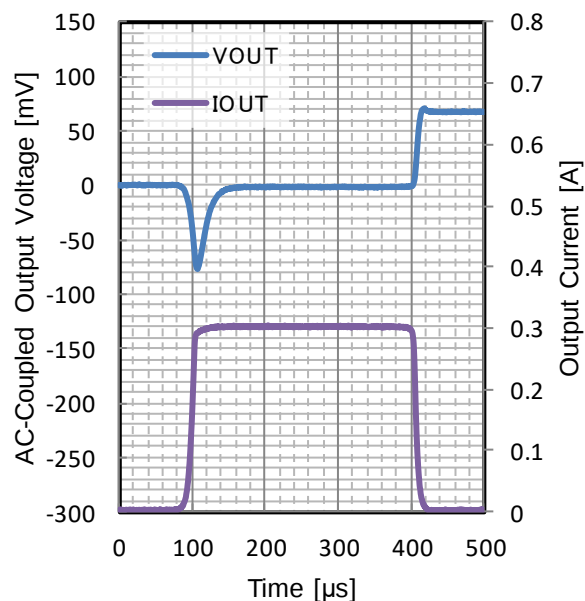
Figure 232. Load Transient
