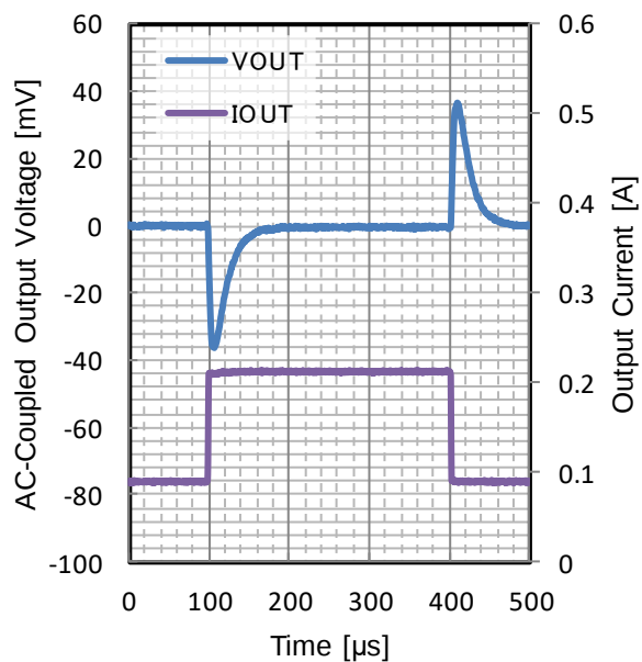
Figure 228. Load Transient
