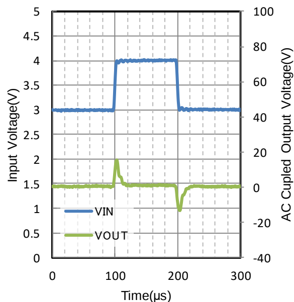
Figure 156. Line Transient
