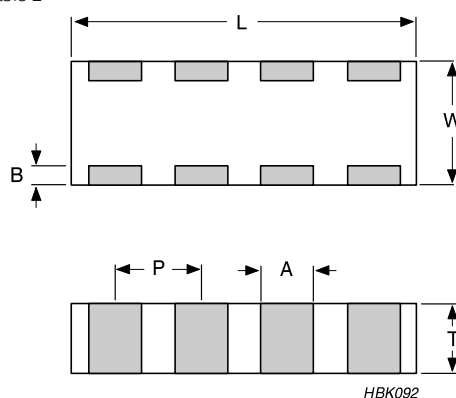
Fig. 3 Surface mounted multilayer ceramic capacitor dimension
