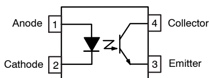
Figure 2. Schematic – FOD817
