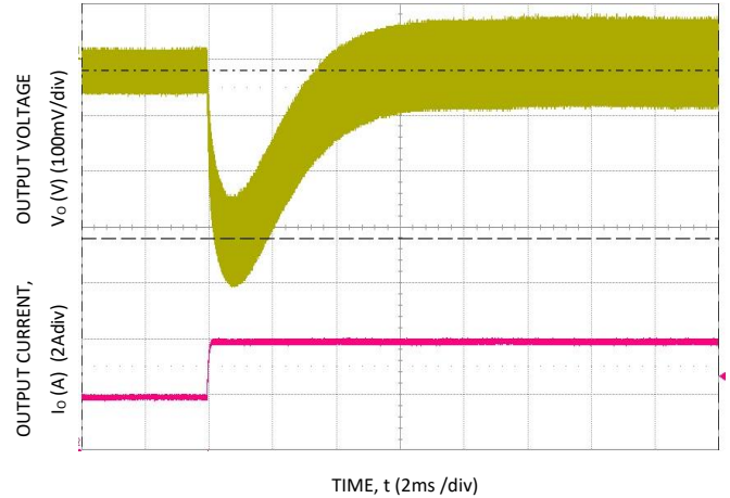
Figure 4. Transient Response to Dynamic Load Change from 50% to 100% at 12Vin, C_{out}=3 \times 10 \mu\text{F} + 220 \mu\text{F} , C_{Tune}=6800\text{pF} , R_{Tune}=30.1\text{k}\Omega
